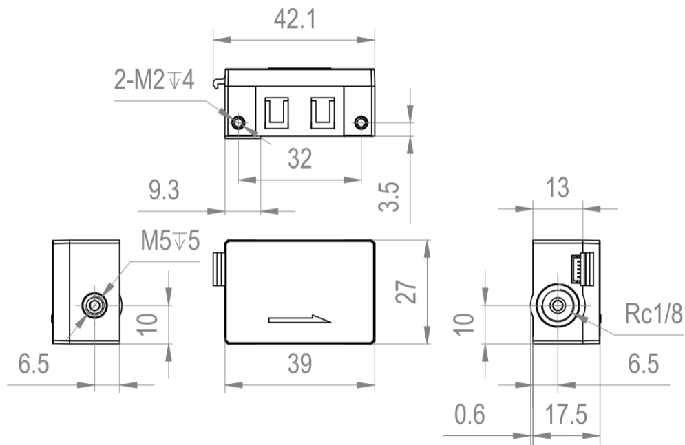
Figure 3.4: FS8003E mechanical dimensions.
