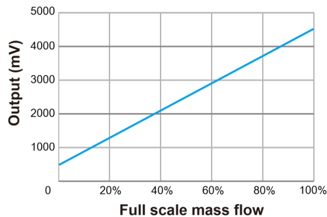
Figure 7.1: The typical analog output of the linearized models: FS8001 and FS8003E.
