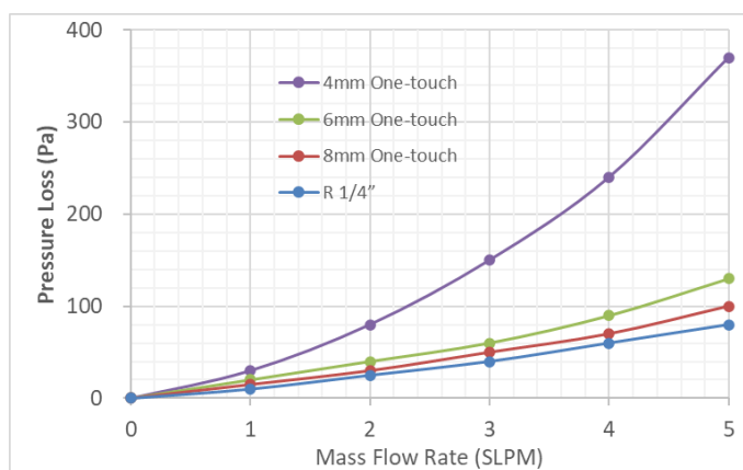
Figure 5.5: MF4003 pressure loss (full scale 2, 3, 4, 5 SLPM)
