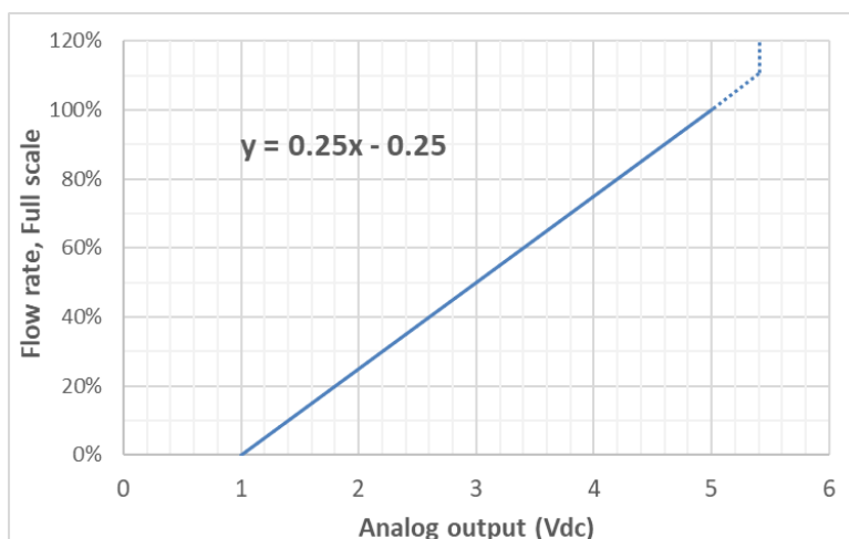
Figure 5.4: MF4000 analog output 1 ~ 5 Vdc
