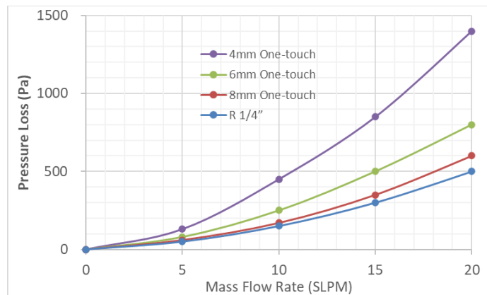
Figure 5.6: MF4008 pressure loss (full scale 10, 20 SLPM)
