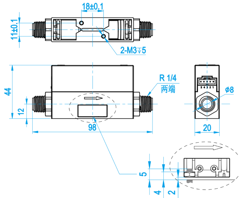
Figure 3.3: MF4000 dimensions with BSPT (R1/4") connectors
