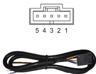
Figure 3.2: MF4000 connection and cable (Part number: SN5-50)
