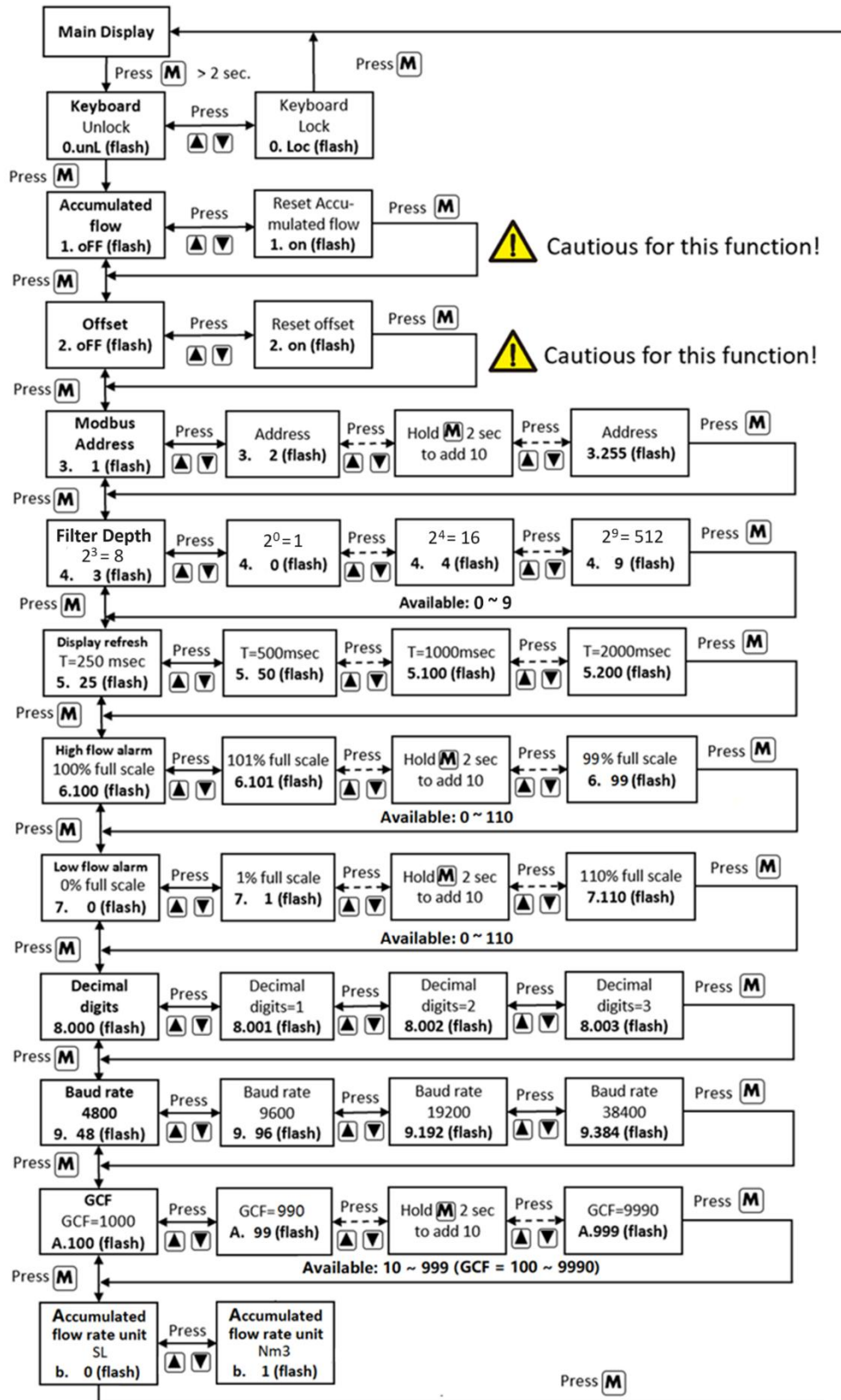
Figure 5.2: MF4000 menu flow chart
