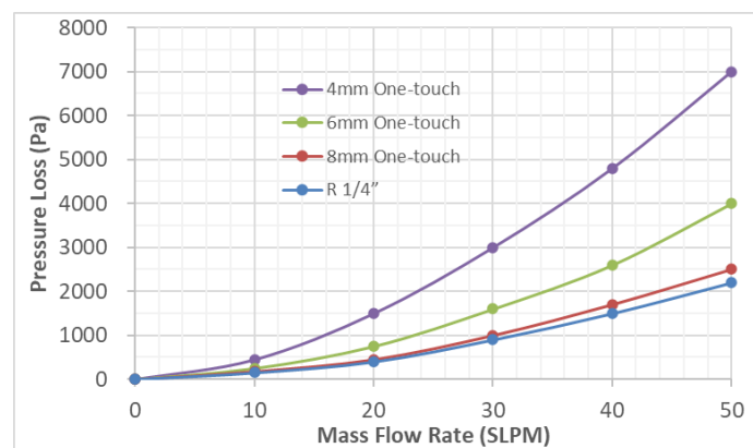
Figure 5.7: MF4008 pressure loss (full scale 30, 40, 50 SLPM)
