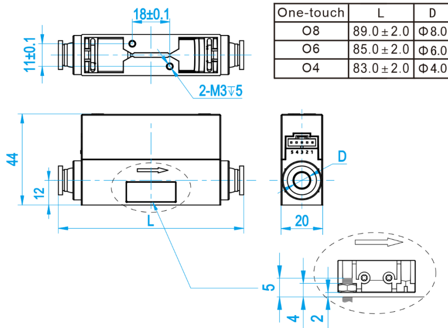
Figure 3.4: MF4000 dimensions with one-touch connectors
