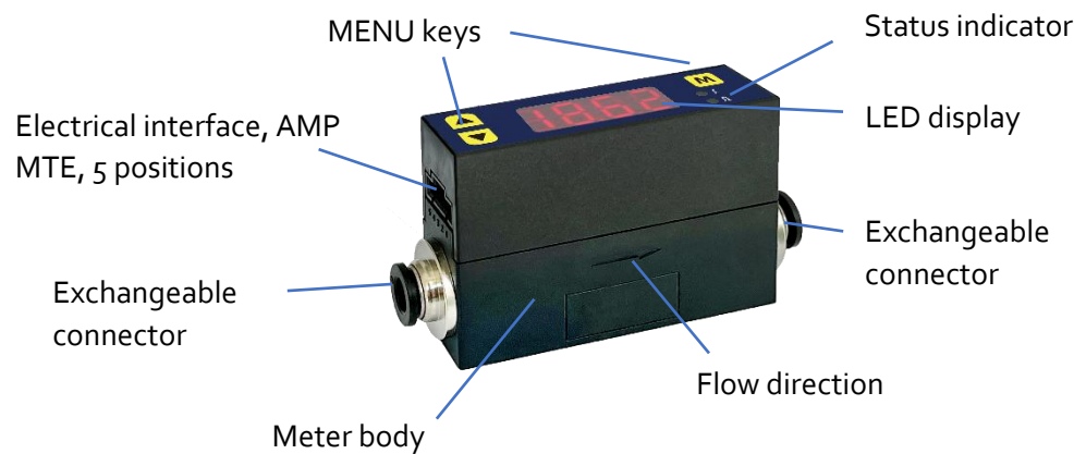
Figure 3.1: MF4000 parts description
